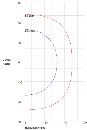
ISOCANDELA CURVES
